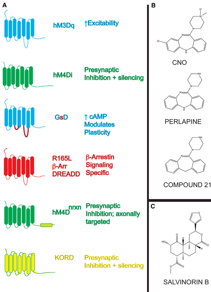
Figure 3. Available DREADDs and Chemical Actuators
