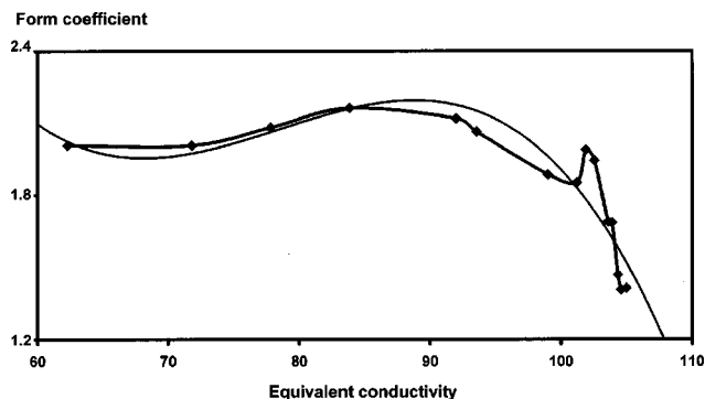
FIG. 6. Dependence of form coefficient on equivalent conductivity [measured in \text{cm}^2 \Omega^{-1} (\text{g.-equiv.})^{-1} ] for KNO 3 is shown in bold line. Approximation of this dependence by the third order polynomial -5 \times 10^{-5} x^3 + 0.013x^2 - x + 27.2 is shown in regular line.
